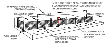
INSTALLATION OF SEDIMENT FENCE N.T.S.
