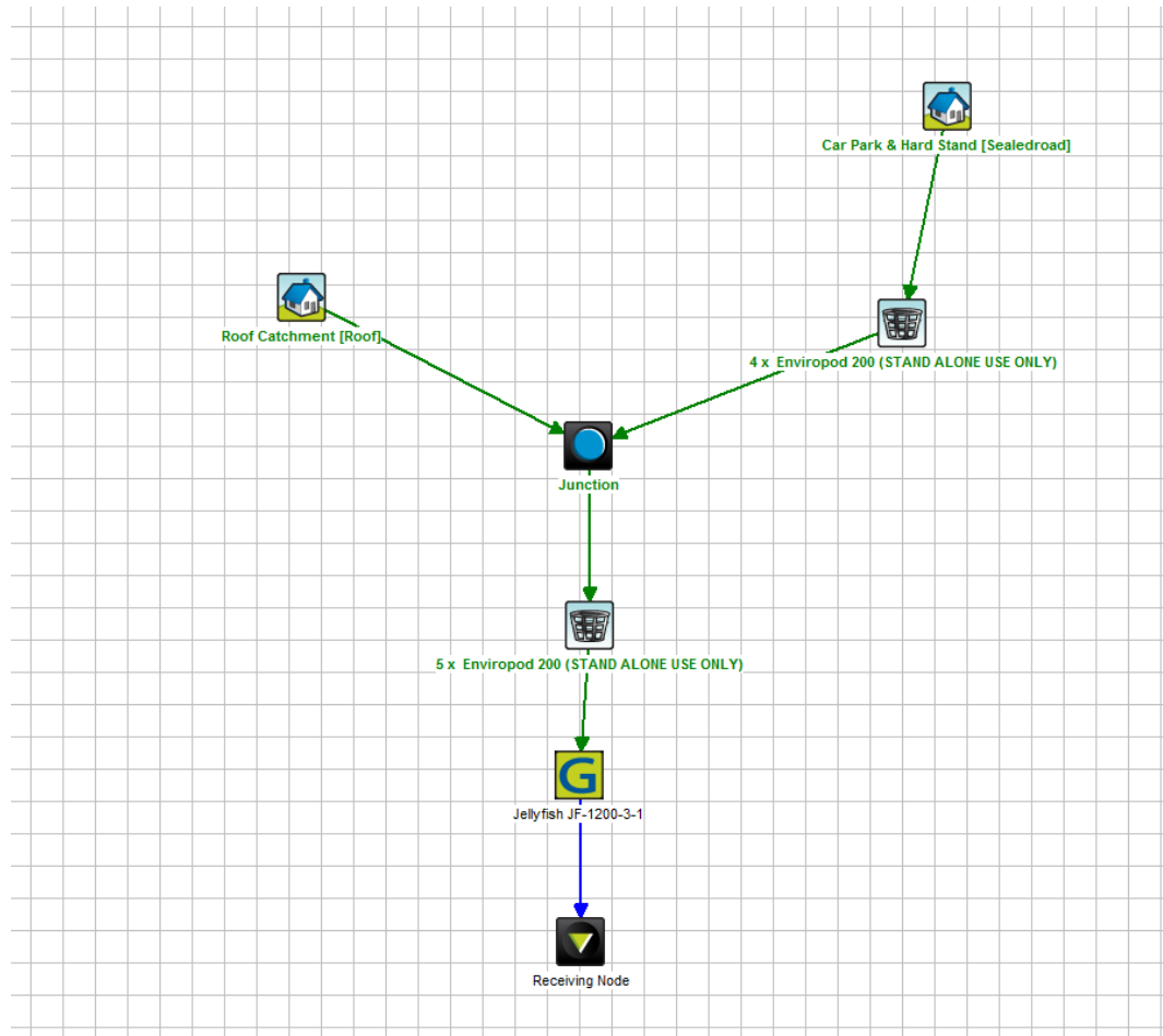
Figure 5 MUSIC Model
